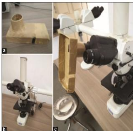
Figure 1: (a) Mobile phone mount made of the cardboard. (b) Nikon microscope. (c) Mount attached to the eye-piece of microscope
